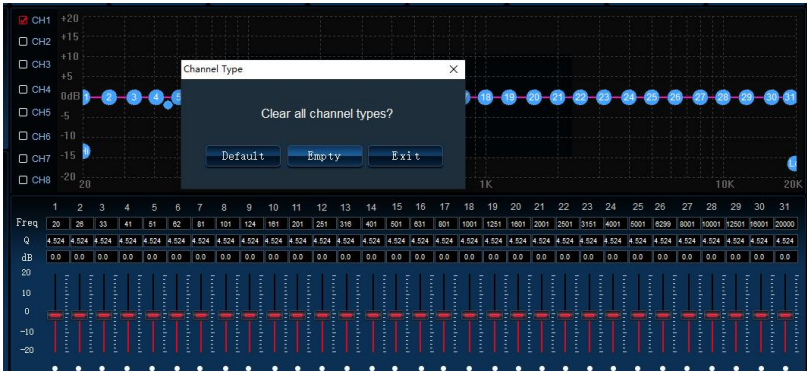
Figure 3.3.4
